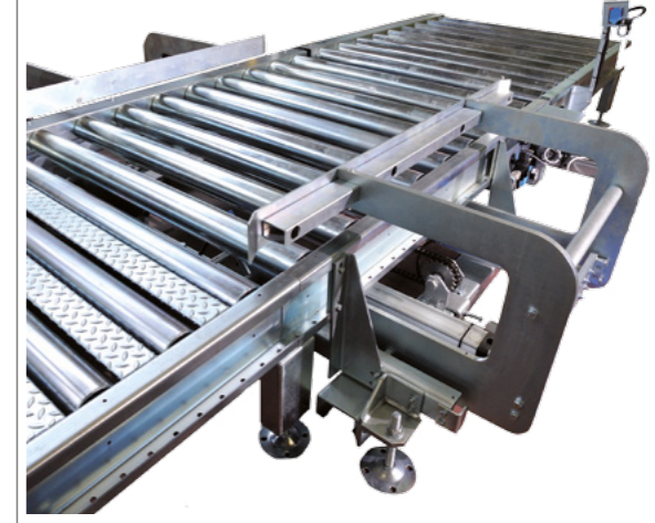
ROTATING PLATFORM WITH CHAINS
