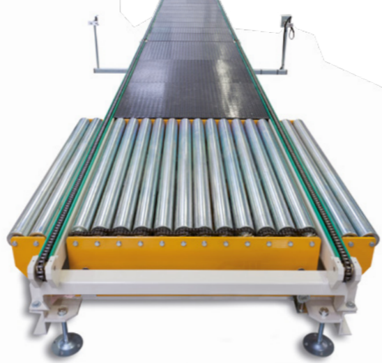
90° PALLET TRANSFER CHAINS AND ROLLERS
