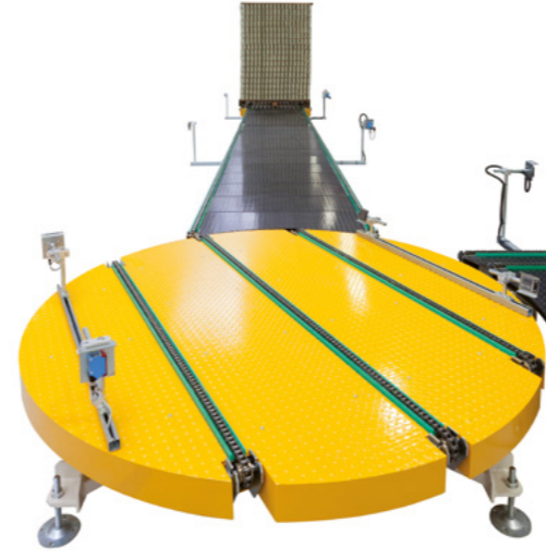
ROTATING PLATFORM WITH CHAINS
